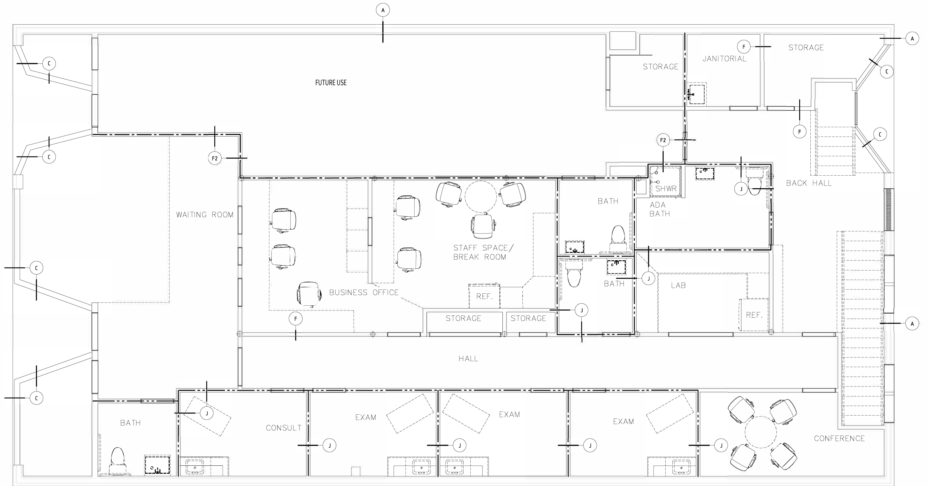
1 PROPOSED MAIN LEVEL RCP \frac{3}{16}'' = 1'-0''
